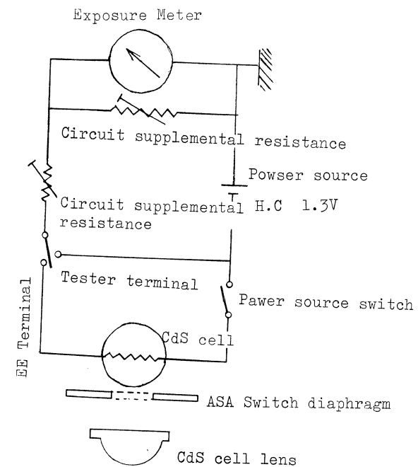
METER CIRCUIT DIAGRAM
