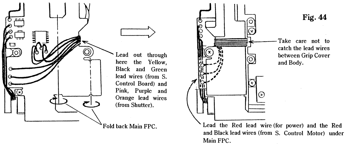
[Chart for Dressing of Lead Wires on Right Side of Body]
