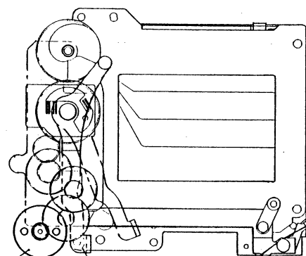
(Shutter Control Mechanism)
