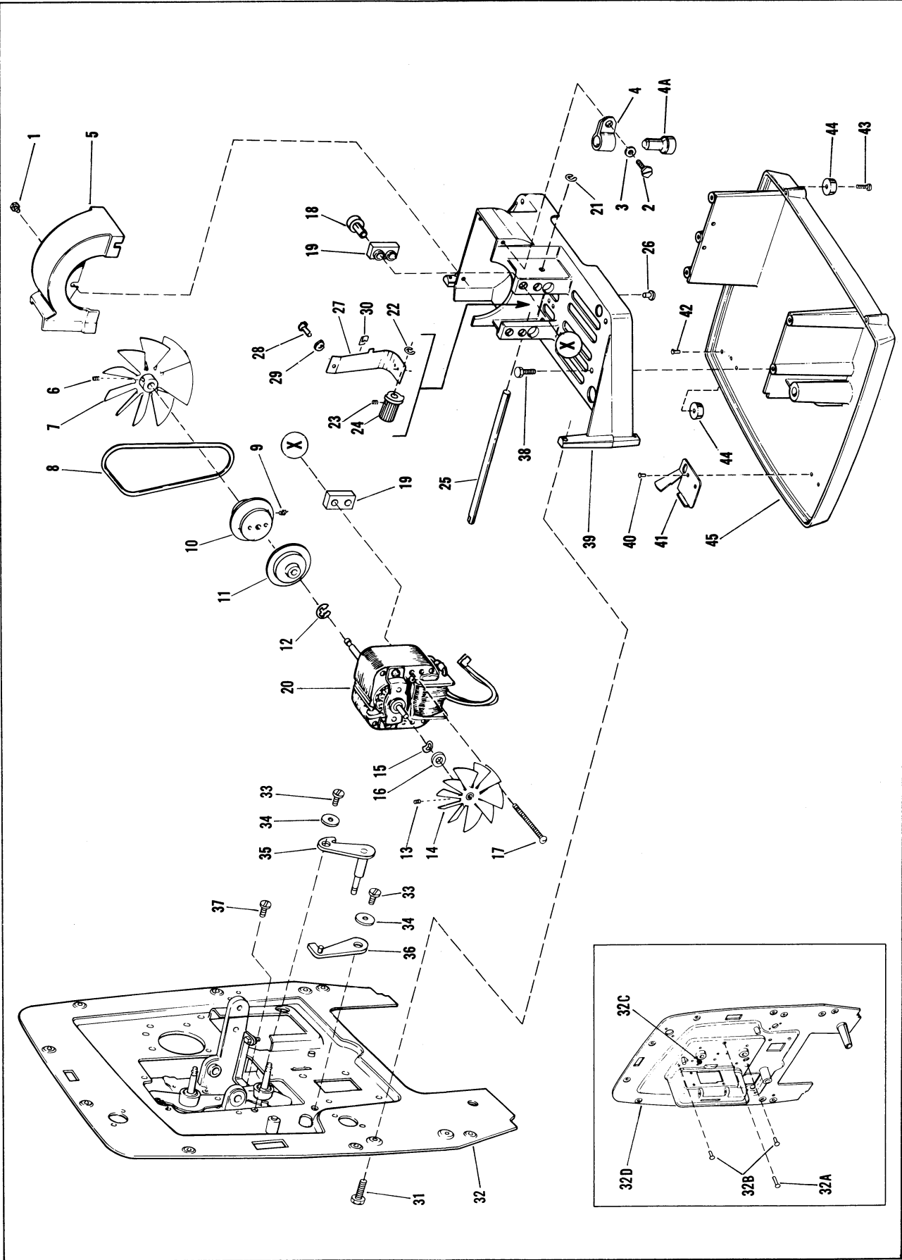
Figure 6. Motor Fans and Base
