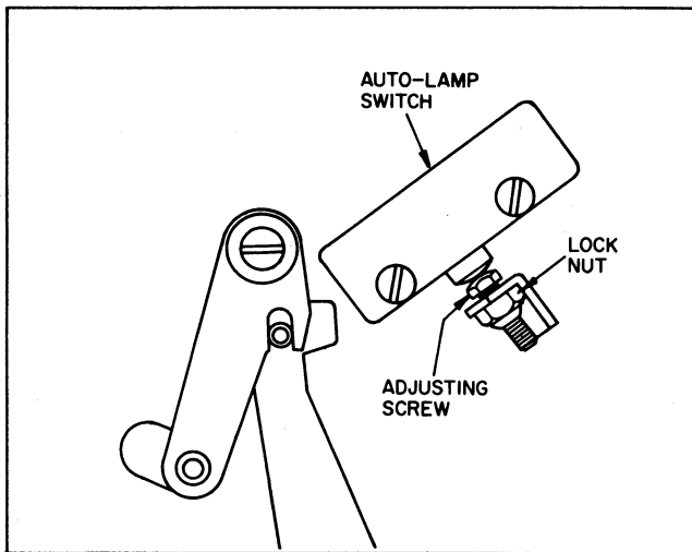
Figure L. Auto-Lamp Switch Adjustment
