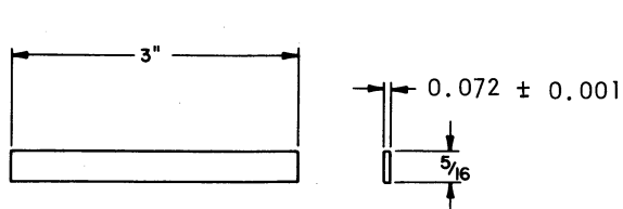
LENS CARRIER SETTING GAGE
