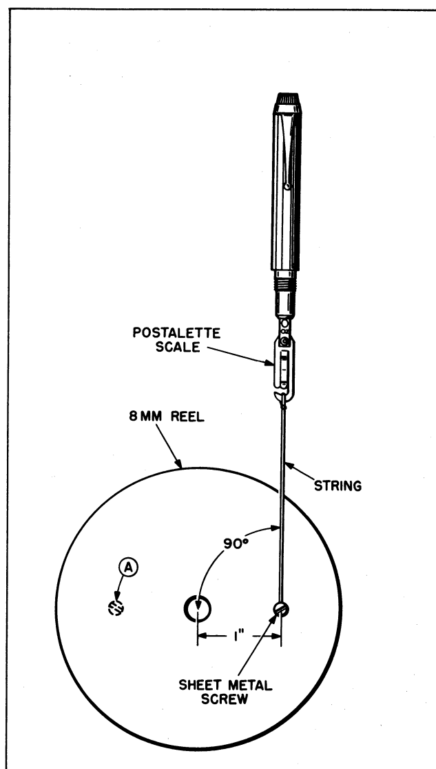
Figure F. Checking Reel Spindle Torque
