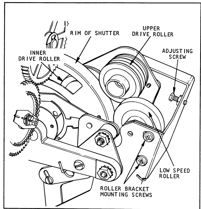
Figure K. Safety Shutter Adjustment
