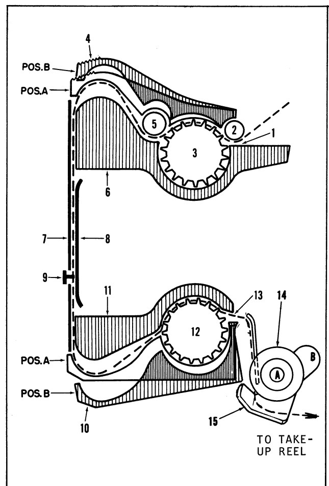
Figure A. Autoload Theory View
