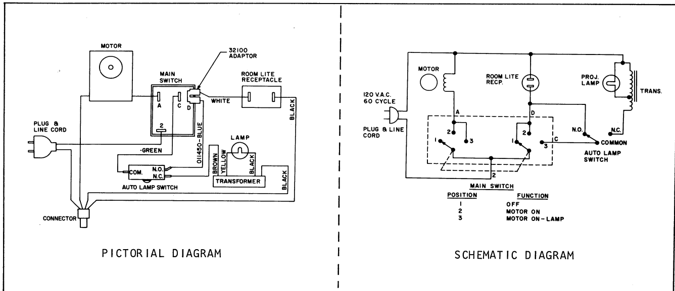
Figure M. Projector Wiring Diagrams
