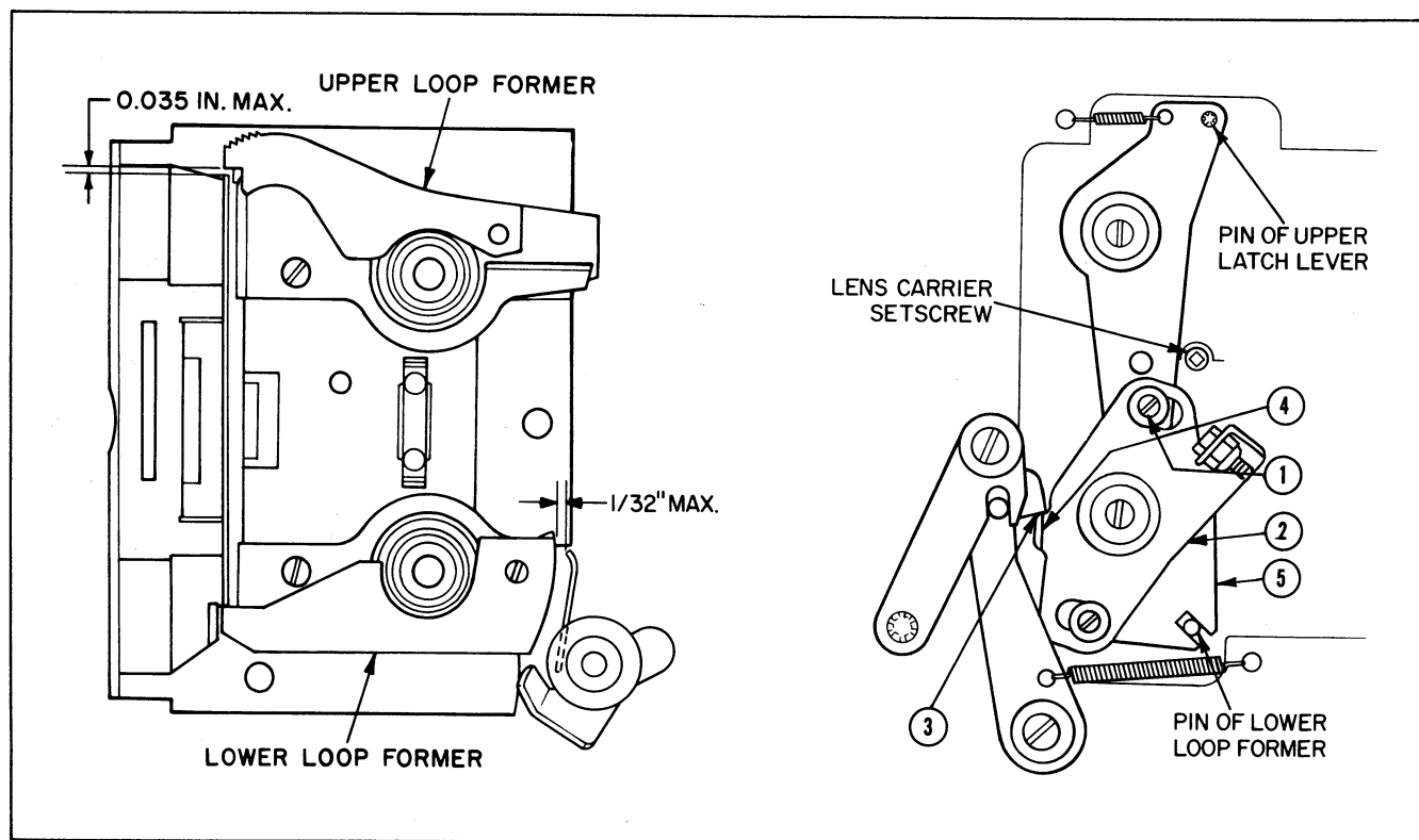
Figure E. Adjusting Trip Levers and Loopformers
