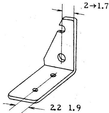
Connecting Lever
