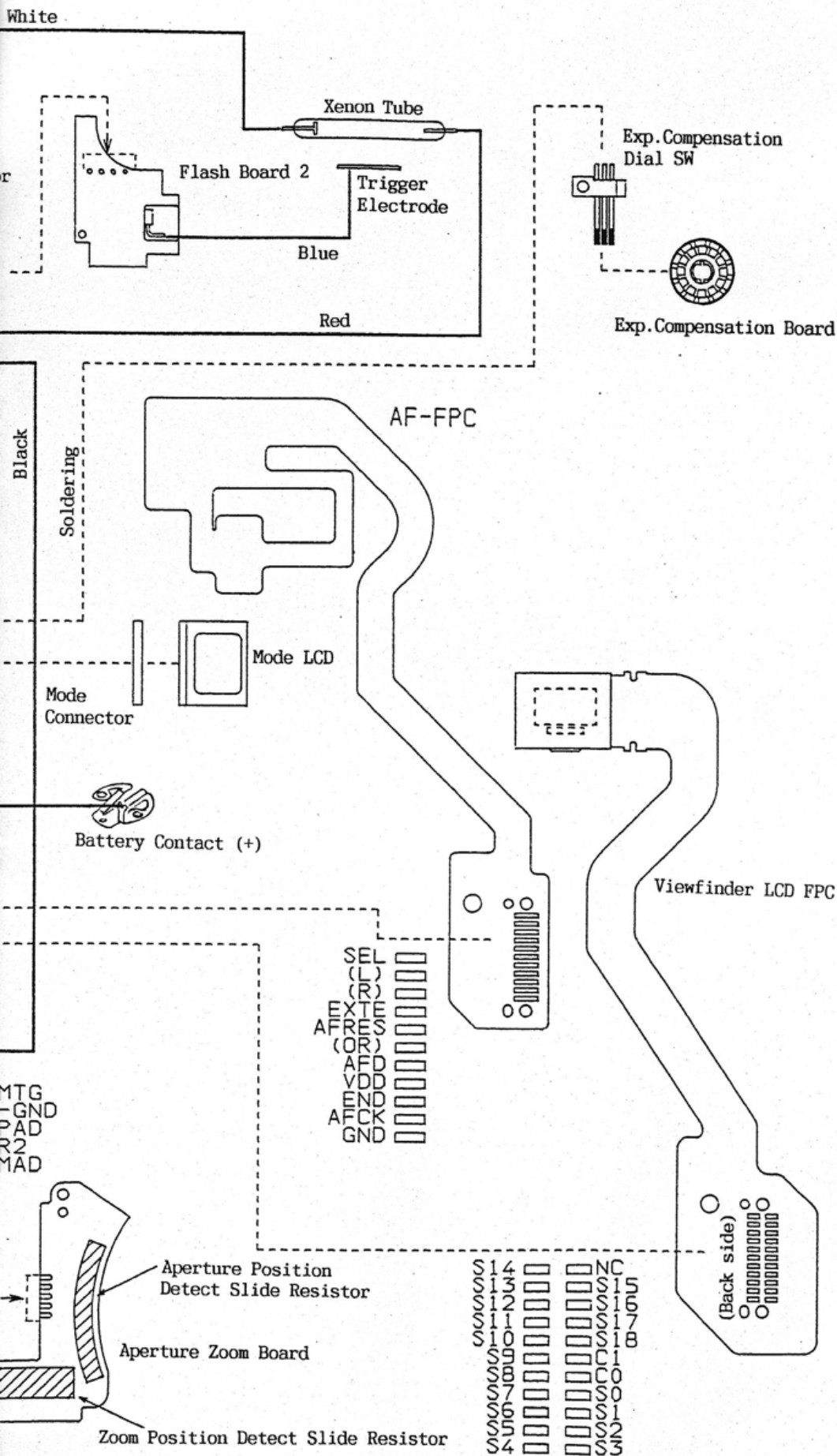
OLD TYPE WIRING DIAGRAM
