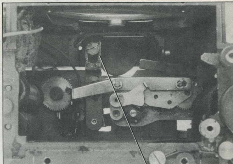
DIAPHRAGM-CLOSING LINK
